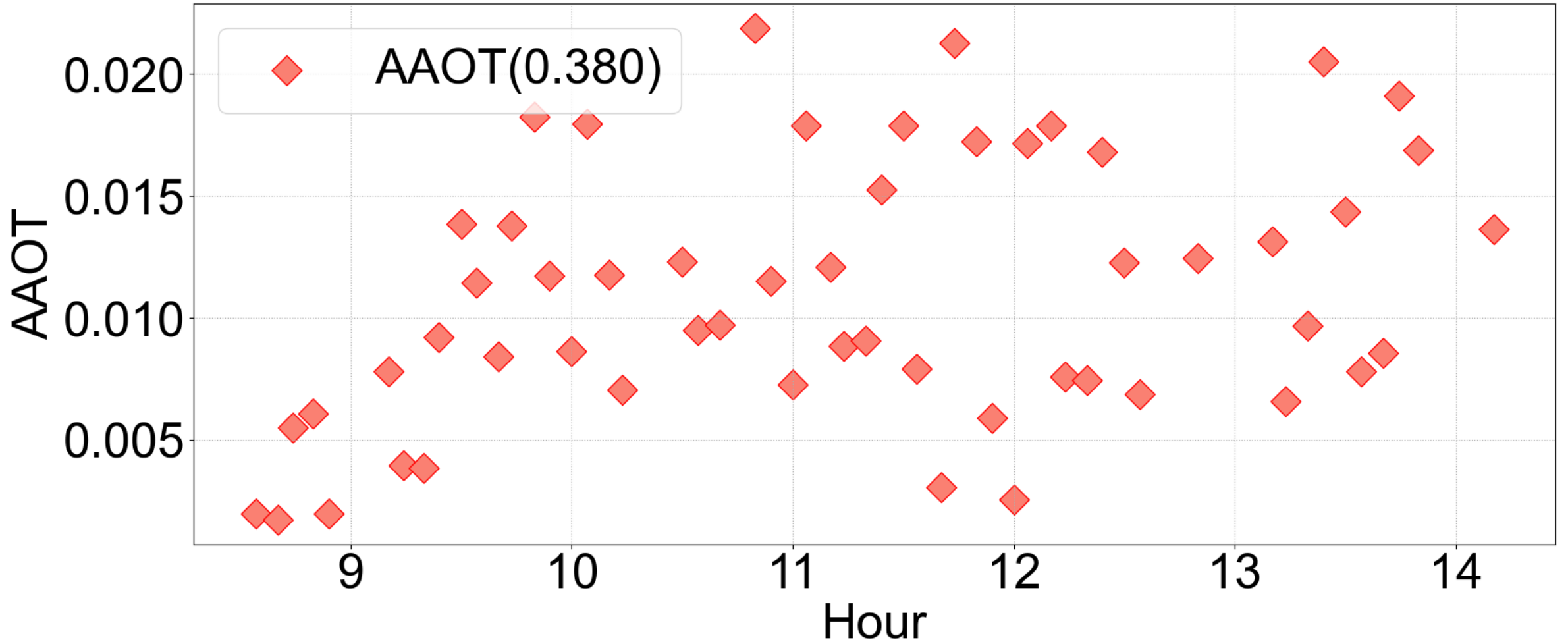
AAOT in Chiba for 2023.11.29
