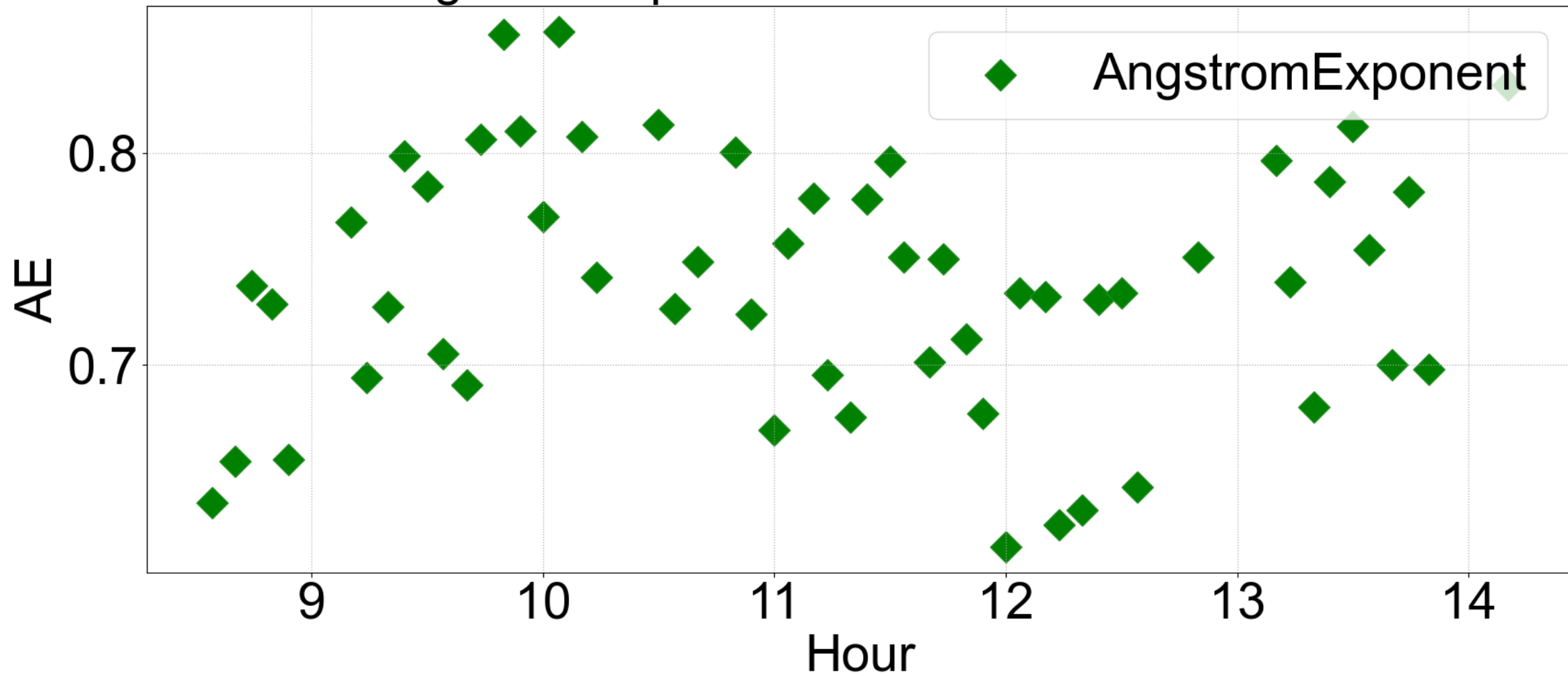
AngstromExponent in Chiba for 2023.11.29
