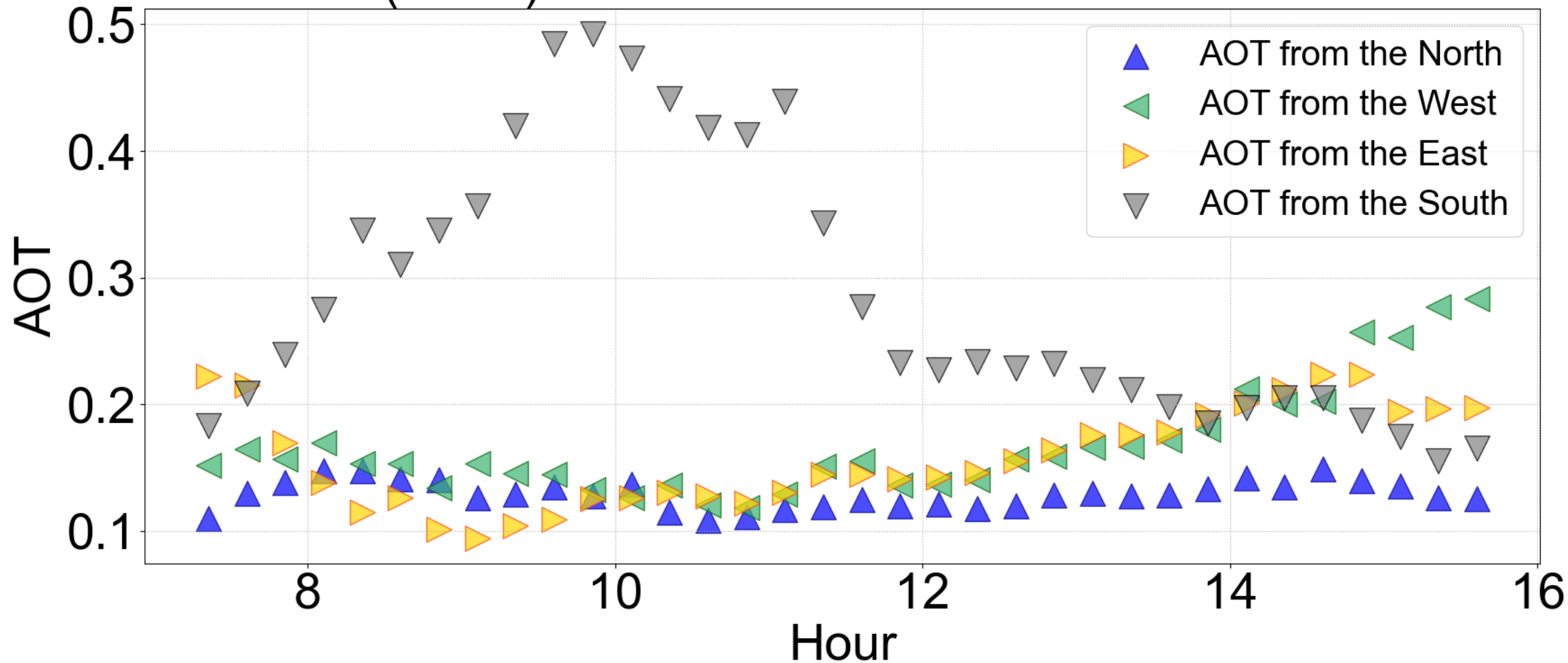
AOT(0.357) of MAX-DOAS in Chiba for 2023.11.29
