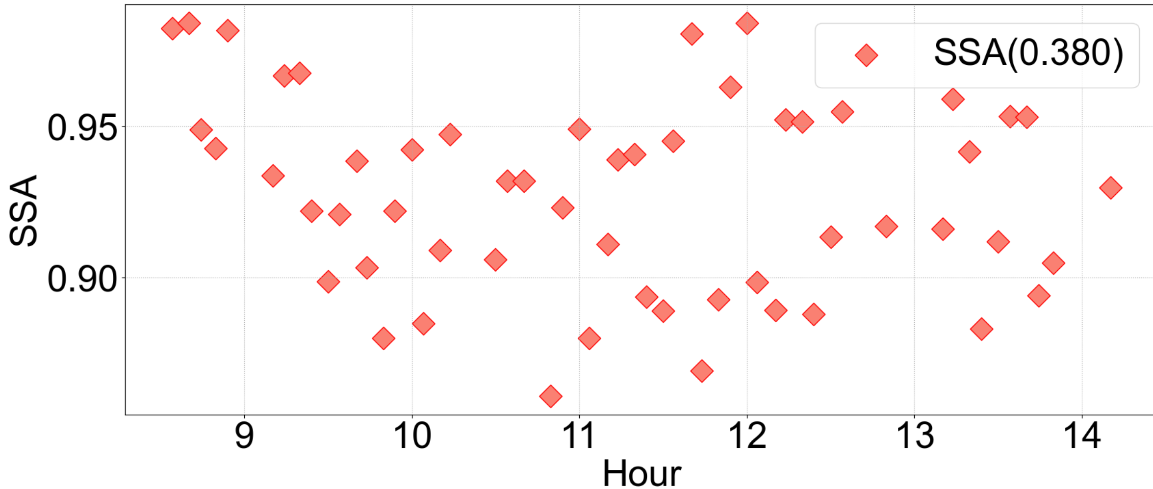
SSA in Chiba for 2023.11.29
